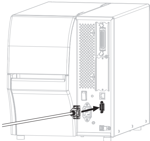
Serial Connector
