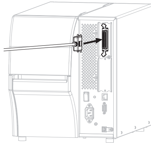
Parallel Connector
